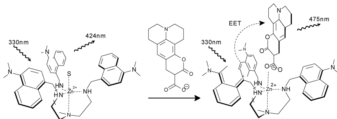
Fig. 38. Electronic energy transfer (EET) from the N,N -dimethylamine-1-naphthalene fragment ( \text{Fl}_1 ) to the dye coumarine-343 ( \text{Fl}_2 ). Coordination of the dye to \text{Zn}^{\text{II}} brings \text{Fl}_1 close enough to \text{Fl}_2 to permit the EET process to occur. Adapted from Ref. [34].
