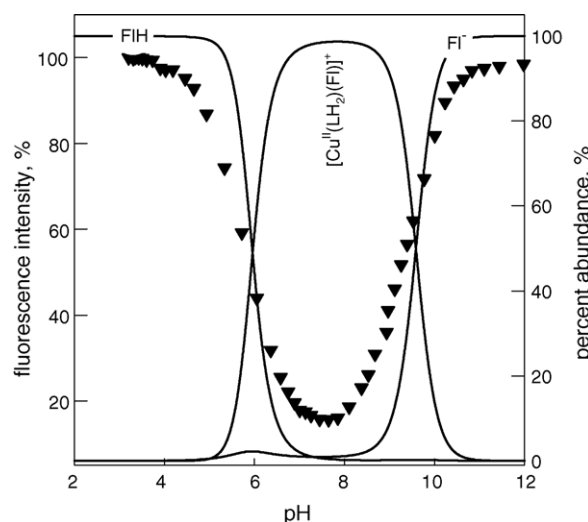
Fig. 30. Full triangles (left vertical axis) indicate the fluorescence intensity, I_{\text{F}} , of a solution 2 \times 10^{-6} M in coumarin-343 ( 28 ) and 4 \times 10^{-4} M in the [\text{Cu}^{\text{II}}(\text{LH}_2)]^{2+}/[\text{Cu}^{\text{II}}(\text{L})] complex ( \text{LH}_2 = \text{31} ). Values of the descending arm of the well-shaped profile refer to the emission band at 490 nm (emitting fragment: undissociated form, FIH); values of the ascending arm refer to the emission band at 471 nm (emitting fragment: dissociated form, \text{FI}^- ). I_{\text{F}} values are normalised. Solid lines (right vertical axis) give the pH dependence of the concentration of FIH, [\text{Cu}^{\text{II}}(\text{LH}_2)(\text{FI})]^+ , and \text{FI}^- , in the same solution. Moving up from pH = 7, fluorescence OFF (bottom of the well) signals that \text{Cu}^{\text{II}} stays in compartment B, fluorescence ON signals that \text{Cu}^{\text{II}} is in compartment A. Adapted from Ref. [31].
