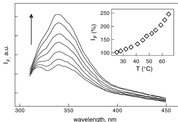
Fig. 40. The emission spectra of a 10^{-6} M solution of \text{Ni}^{\text{II}}(\text{36})(\text{CF}_3\text{SO}_3)_2 in MeCN, recorded over the 27–65 °C temperature range: on increasing temperature, the fluorescence intensity, I_F , grows. The I_F vs. temperature plot (inset) provides the calibration curve of the molecular fluorescent thermometer. Adapted from Ref. [36].
