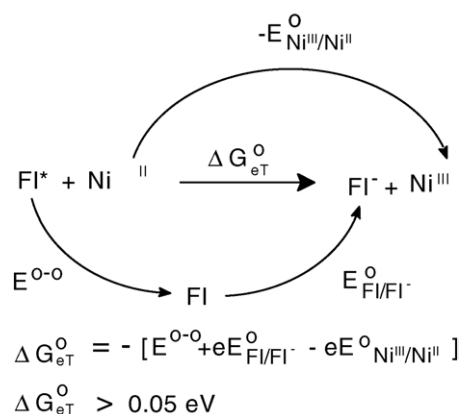
Fig. 6. Thermodynamic cycle for evaluating the free energy change \Delta G_{eT}^{\circ} associated with the intramolecular photoinduced electron transfer in the [Ni^{II}(4)]^{2+} . E^{O-O} = 3.80 \text{ eV} ; E^{\circ}(FI/FI^-) \leq -3.10 \text{ V} , since no peaks were observed in the cathodic scan in voltammetry experiments until solvent discharge; E^{\circ}(Ni^{III}/Ni^{II}) = 0.75 \text{ V} . The coulombic term was considered negligible under the present circumstances.
