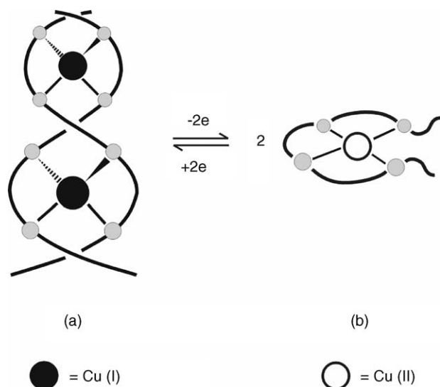
Fig. 17. The disassembling–assembling of a dimetallic helicite, driven by the \text{Cu}^{\text{I}}/\text{Cu}^{\text{II}} redox change. \text{Cu}^{\text{I}} likes tetrahedral coordination and favours the assembling of the bis-bidentate ligand to give a double helix (a). Such an arrangement is not congruent with the square coordination required by \text{Cu}^{\text{II}} , whose formation induces disassembling of the dinuclear helicite and formation of two mononuclear complexes (b). Reproduced from Ref. [26], with permission of the copyright owners.
