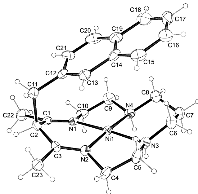
Fig. 9. ORTEP diagram of the [Ni II L] 2+ complex: L = 5,7-dimethyl-6-naphthalen-2-ylmethyl-1,4,8,11-tetraaza-cyclotetradeca-4,7-diene [18]. The naphthalene fragment is located above the tetra-aza-macrocyclic ring, acting as a roof for the Ni II ion. Such an arrangement may be due the establishment of interactions between the nitrogen atoms of the macrocycle and the aromatic subunit. Reproduced from Ref. [18], with permission of the copyright owners.
