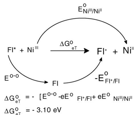
Fig. 5. Thermodynamic cycle for evaluating the free energy change \Delta G_{\text{eT}}^\circ associated with the intramolecular photoinduced electron transfer in the nickel(III) complex of 4 . E^{0-0} = 3.80 eV; E^0(\text{Fl}^+/\text{Fl}) = 1.45 V (irreversible peak); E^0(\text{Ni}^{\text{III}}/\text{Ni}^{\text{II}}) = 0.75 V. The coulombic term was considered negligible under the present circumstances. Reproduced from Ref. [13], with permission of the copyright owners.
