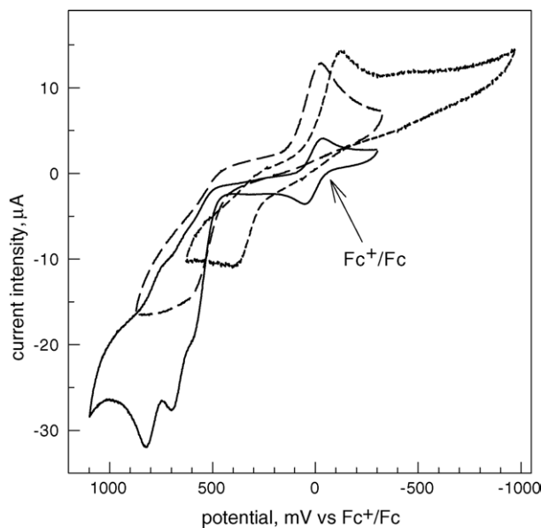
Fig. 22. Cyclic voltammety profiles for [\text{Cu}_2^{\text{I}}(\mathbf{26})_2]^{2+}/[\text{Cu}^{\text{II}}(\mathbf{26})]^{2+} (long dash) and [\text{Cu}_2^{\text{I}}(\mathbf{27})_2]^{2+}/[\text{Cu}^{\text{II}}(\mathbf{27})]^{2+} (short dash), in MeOH 0.1 M [\text{Bu}_4\text{N}]\text{ClO}_4 ; potential scan rate: 100 \text{ mV s}^{-1} . The solid line refers to a solution of coumarine 343, to which a small amount of ferrocene had been added, as an internal standard. Reproduced from Ref. [26] with permission of the copyright owners.
