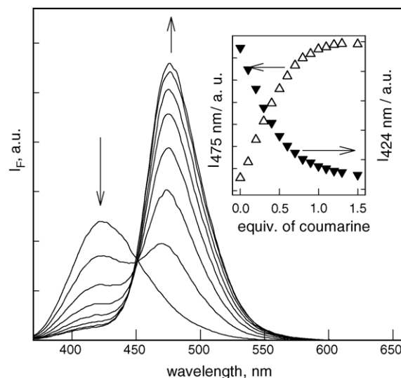
Fig. 37. Emission spectra of an ethanolic solution of [\text{Zn}^{\text{II}}(\mathbf{35})]^{2+} , when titrated with a standard solution of coumarine-343 ( 28 ). The band at 424 nm ( N,N -dimethylamine-1-naphthalene fragment) decreases, while the band at 475 nm (coumarine-343) increases, indicating the occurrence of an electronic energy transfer process. Adapted from Ref. [34].
