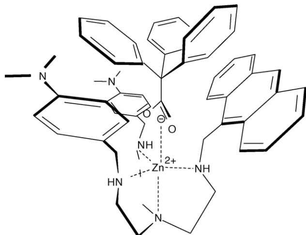
Fig. 36. The proposed structure of the [\text{Zn}^{\text{II}}(\mathbf{34})(\text{TPA})]^+ adduct (TPA = 1,1,1-triphenylacetate). The bulky carboxylate anion stops the electron transfer from one of the N,N -dimethylaniline substituents to the photoexcited anthracene fragment, which can now release its full fluorescence.
