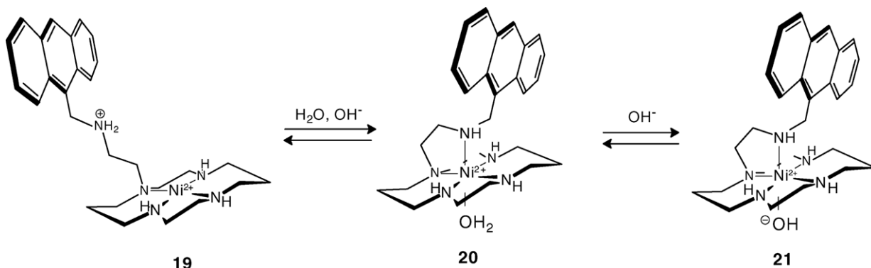
Fig. 13. pH-controlled movement of the fluorescent pendant arm in the \text{Ni}^{\text{II}} scorpionate complex of ligand 18 . Adapted from Ref. [21].
