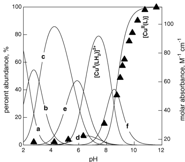
Fig. 29. Percent concentration of the species present at the equilibrium in a solution containing equimolar amounts of 31 (=LH 2 ) and Cu 2+ (left vertical axis); profiles a , b , c , and d refer to the variously protonated forms of LH 2 (from LH 6 4+ to LH 3 + ). Profile e refers to the metal containing protonated species [Cu II (LH 3 )] 3+ . Profile f refers to the metal containing species [Cu II (LH 2 )(OH)] + . Filled triangles give the molar absorbance of d–d band ( \lambda_{\text{max}} = 502 \text{ nm} ) of the [Cu II (L)] complex (right vertical axis). Adapted from Ref. [31].
